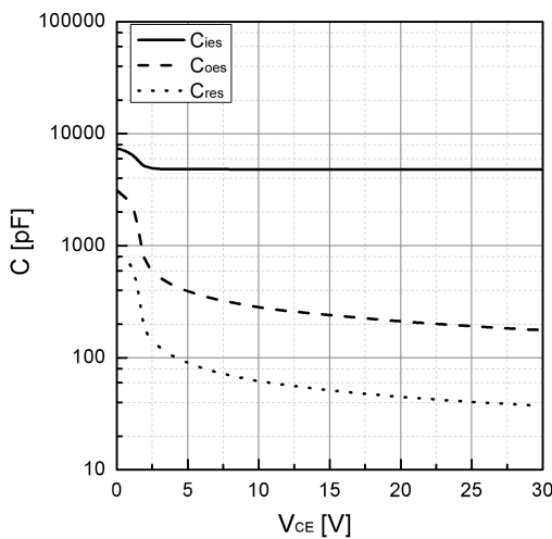
Fig 17. Typical capacitance as a function of V_{CE} ( f=1\text{Mhz} , V_{GE}=0\text{V} )
